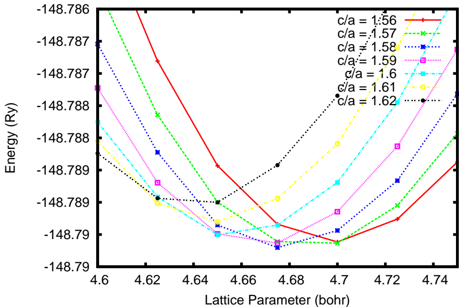
Energy vs Lattice Parameter for hcp Cobalt
